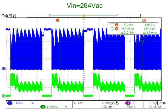
264Vac CH3:Vds CH4:IL
