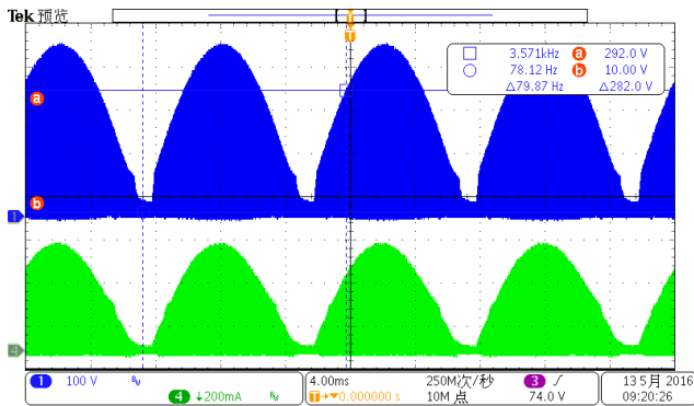
CH3:Vds CH4:Ics
