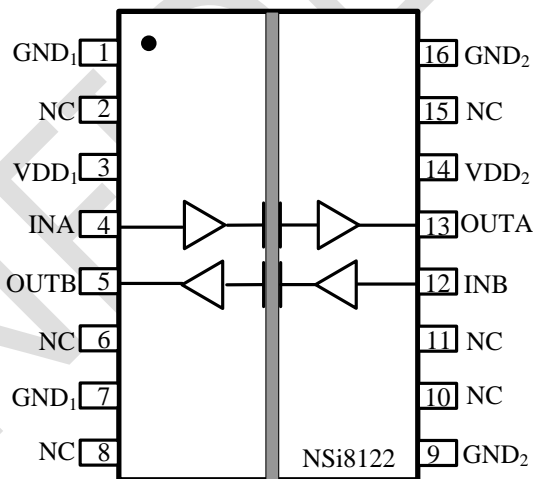
Figure 6.7 NSi8122W Package
