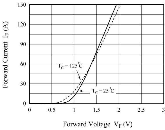
Fig 17. Forward Characteristics
