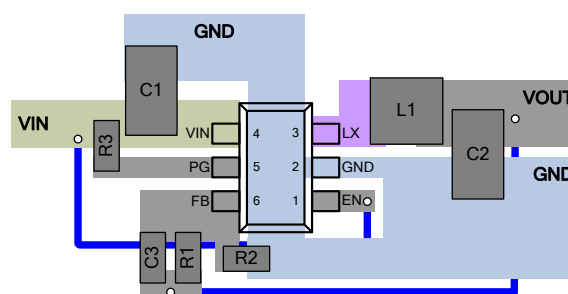
Figure 17. Recommended Layout Diagram
