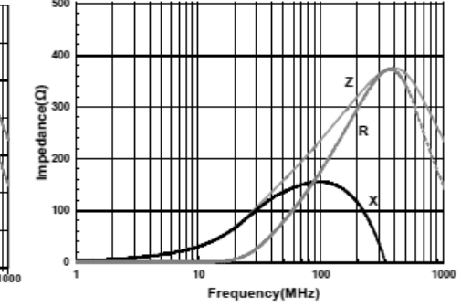
CMBH1005S221JSP
