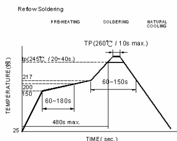
Reflow times: 3 times max.
