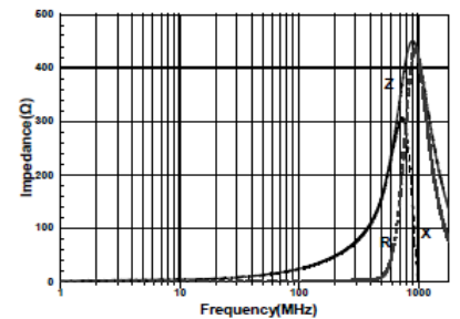
CMBM1608G300JSP
