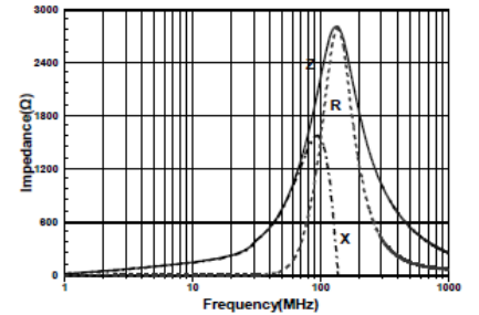
CMBM1608K222BSP
