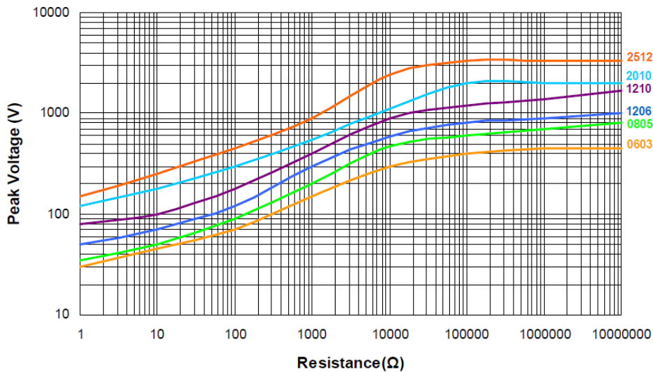
10/700us Lightning Surge(*) RPC-HP (High Power) all tolerances RPC (Standard Power) tolerances of 0.5% and 1%
