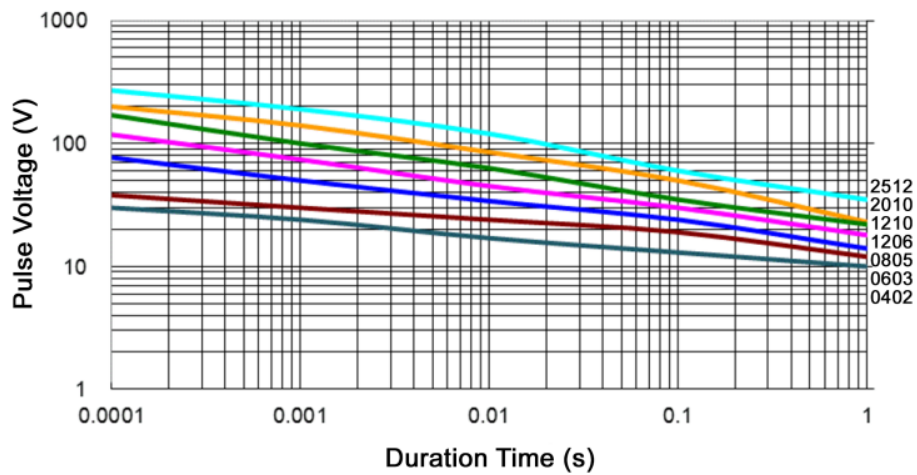
Pulse Voltage (100 Ohm) RPC-HP (High Power) all tolerances RPC (Standard Power) tolerances of 0.5% and 1%
