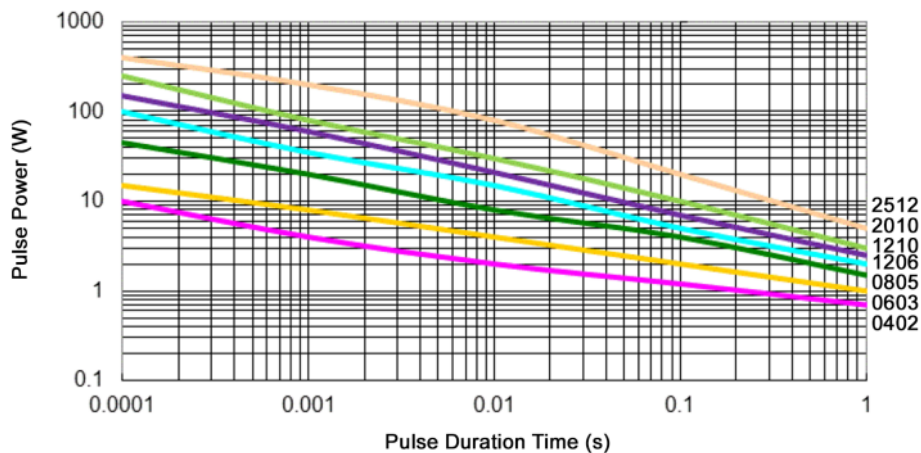
Continuous Pulse Power (100 Ohm) RPC-HP (High Power) all tolerances RPC (Standard Power) tolerances of 0.5% and 1%
