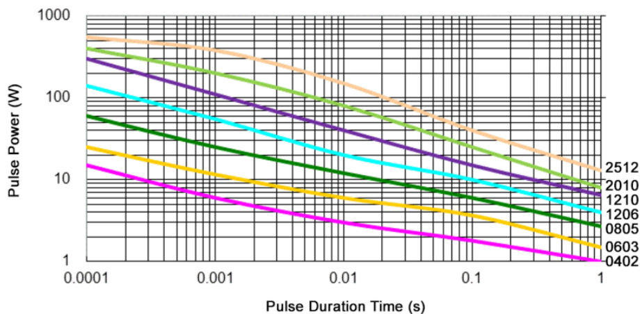
Single Pulse Power (100 Ohm) RPC-HP (High Power) all tolerances RPC (Standard Power) tolerances of 0.5% and 1%
