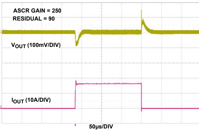
FIGURE 12. 12V IN TO 1V OUT TRANSIENT RESPONSE, f_{SW} = 533kHz , C_{OUT} = 4 \times 100\mu F CERAMIC + 2x470µF POSCAP
