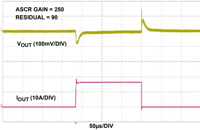
FIGURE 10. 5V IN TO 1V OUT TRANSIENT RESPONSE, f_{SW} = 533kHz , C_{OUT} = 4 \times 100\mu F CERAMIC + 2x470µF POSCAP
