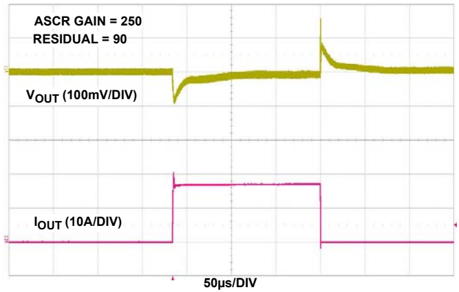
FIGURE 11. 5V IN TO 1.8V OUT TRANSIENT RESPONSE, f_{SW} = 615kHz , C_{OUT} = 3 \times 100\mu F CERAMIC + 2x470µF POSCAP
