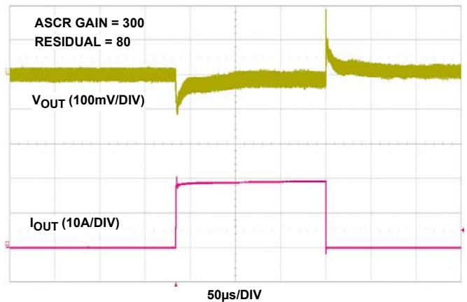
FIGURE 15. 12V IN TO 5V OUT TRANSIENT RESPONSE, f_{SW} = 727kHz , C_{OUT} = 3 \times 100\mu F CERAMIC + 2x470µF POSCAP
