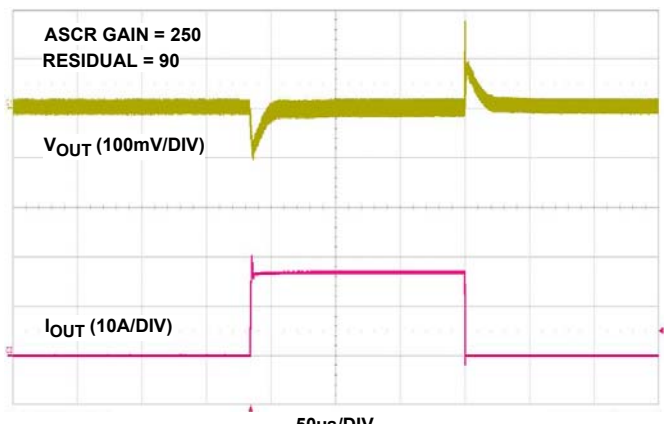
FIGURE 13. 12V IN TO 1.8V OUT TRANSIENT RESPONSE, f_{SW} = 615kHz , C_{OUT} = 3 \times 100\mu F CERAMIC + 2x470µF POSCAP
