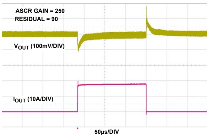
FIGURE 14. 12V IN TO 3.3V OUT TRANSIENT RESPONSE, f_{SW} = 615kHz , C_{OUT} = 3 \times 100\mu F CERAMIC + 2x470µF POSCAP
