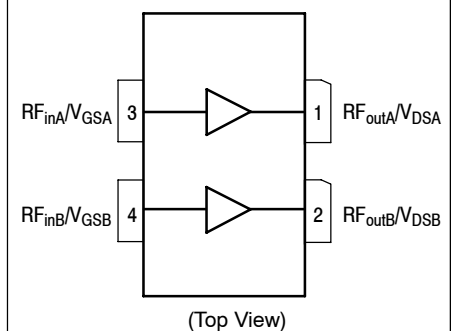
Figure 1. Pin Connections
