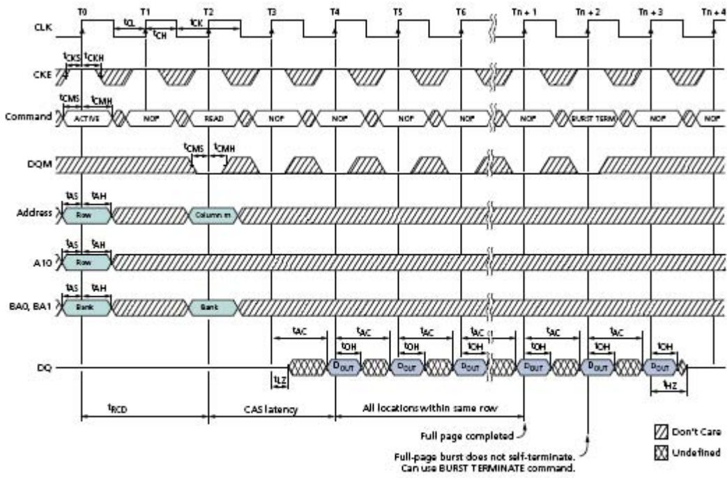
Figure 22: READ Continuous Page Burst
