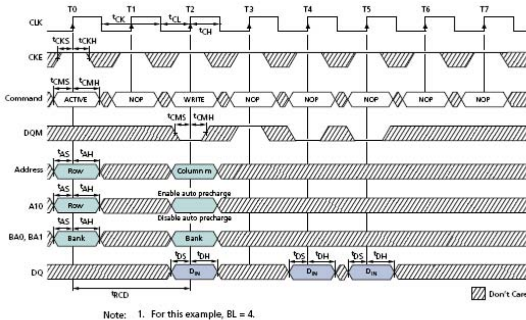
Figure 32: WRITE – DQM Operation
