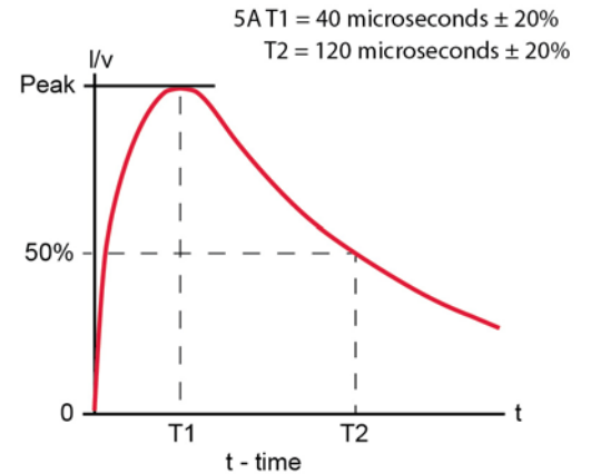
FIGURE 9 – Waveform 5A
