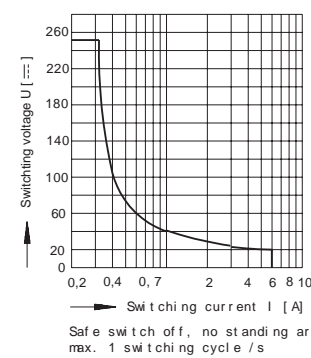
Maximum switching power curve
