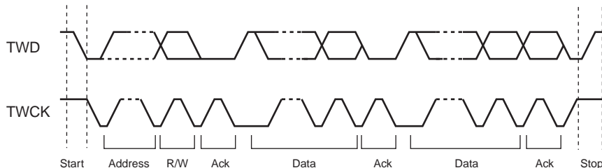
Figure 32-4. Transfer Format
