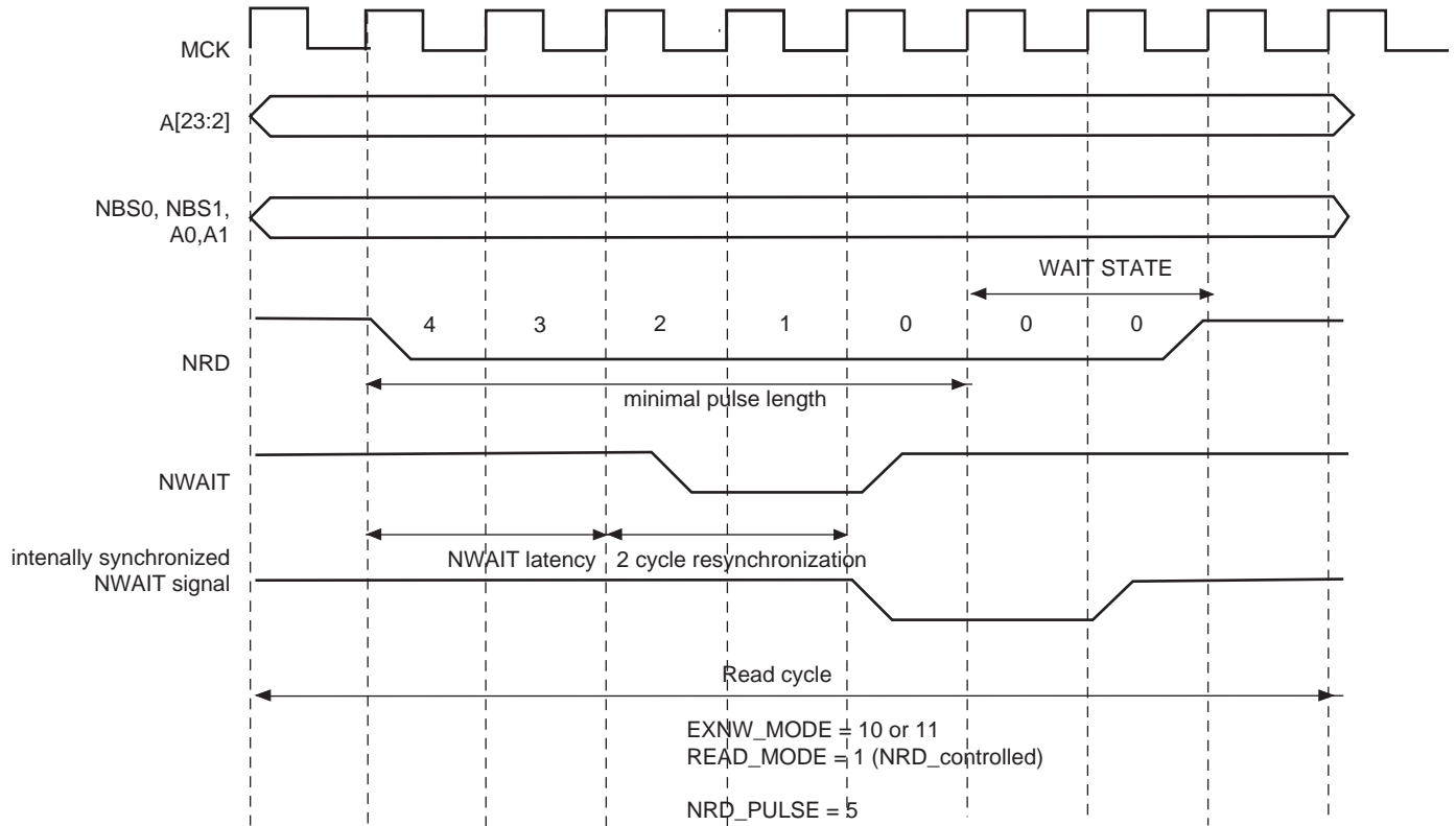
Figure 24-27. NWAIT Latency
