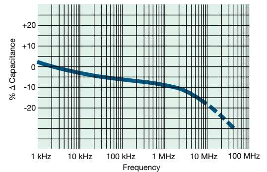
\Delta Capacitance vs. Frequency
