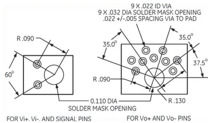
SMT Recommend Pad Layout (Component Side View)
