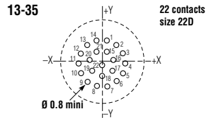
22 contacts size 22D
