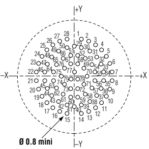
79 contacts size 22D
