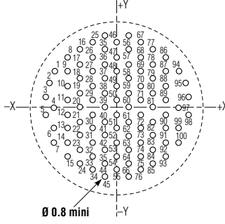
100 contacts size 22D
