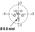
6 contacts size 22D
