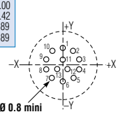
13 contacts size 22D
