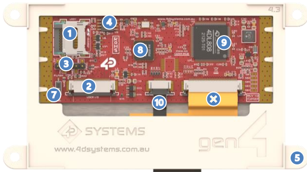
Represents gen4-uLCD-xxP4/P4T/P4CT models
