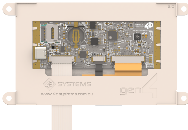
FFC Cable - Under Plastics
