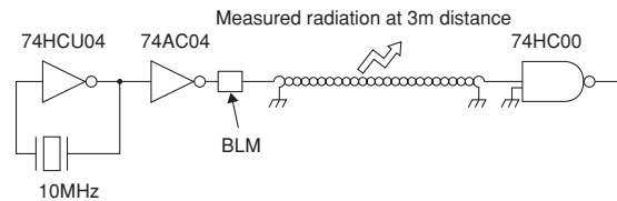
Testing Circuit
