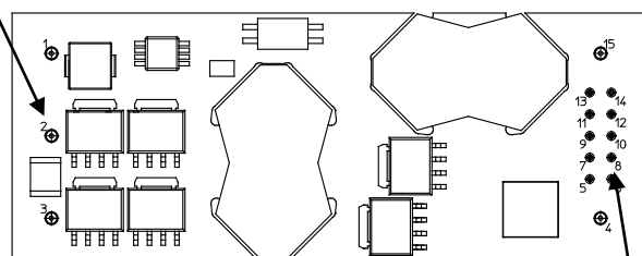
Pin 5 for measurement of minimum pin (solder joint) temperature, T_{PIN}
