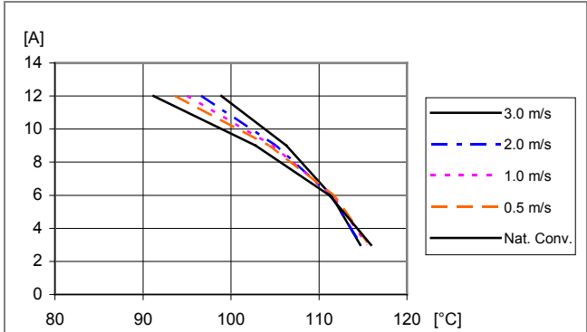
Available load current vs. ambient air temperature and airflow at V_O=1.0\text{ V} , V_I=12\text{ V} . See Thermal Consideration section.
