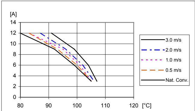
Available load current vs. ambient air temperature and airflow at V_O=5.0\text{ V} , V_I=12\text{ V} . See Thermal Consideration section.
