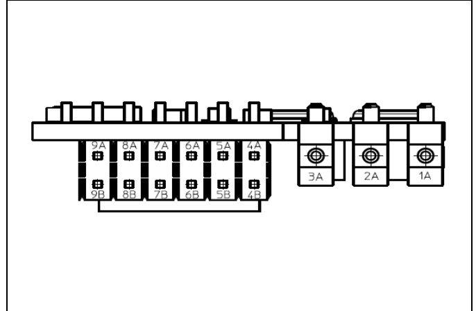
Pin layout, bottom view (component placement for illustration only).
