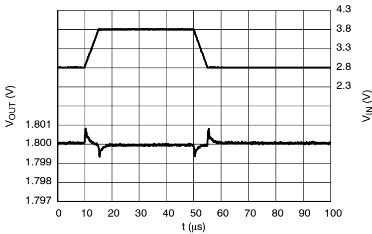
Figure 36. Line Transients, 1.8 V Version, t_{\text{R}} = t_{\text{F}} = 5 \mu\text{s} , I_{\text{OUT}} = 30 \text{ mA}
