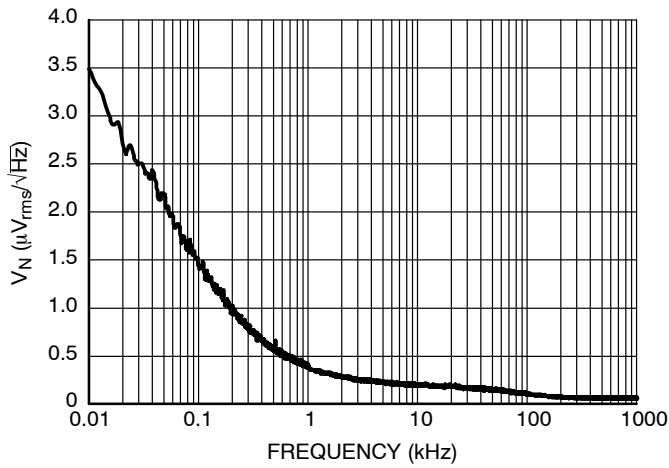
Figure 33. Output Voltage Noise, 2.8 V Version, V_{\text{IN}} = 3.8 \text{ V}
