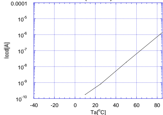
Standby Current vs. Temperature ( V^+=6V )
