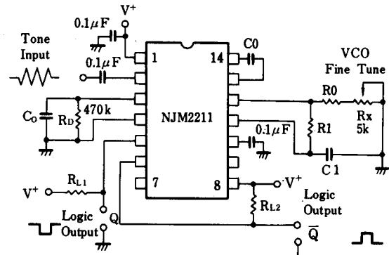
Figure 4. Tone Detection
