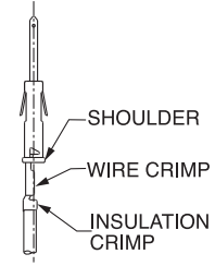
Figure 5 - Unacceptable, Front View
