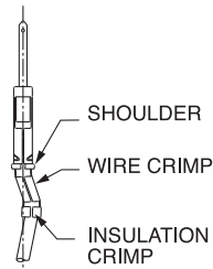
Figure 4 - Correct, Front View
