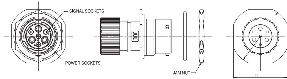
Panel Cutout
