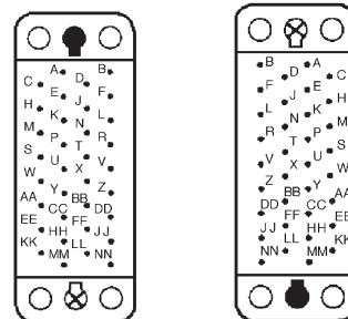
Plug Receptacle
