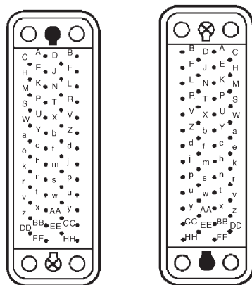
Plug Receptacle
