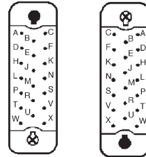
Plug Receptacle
