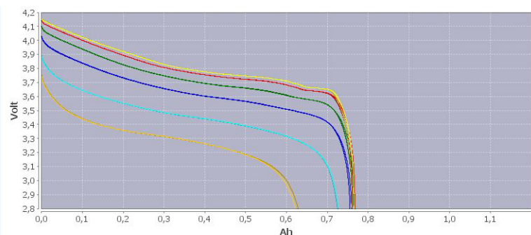
Discharge characteristics of the cell ICR14650-110PCM
