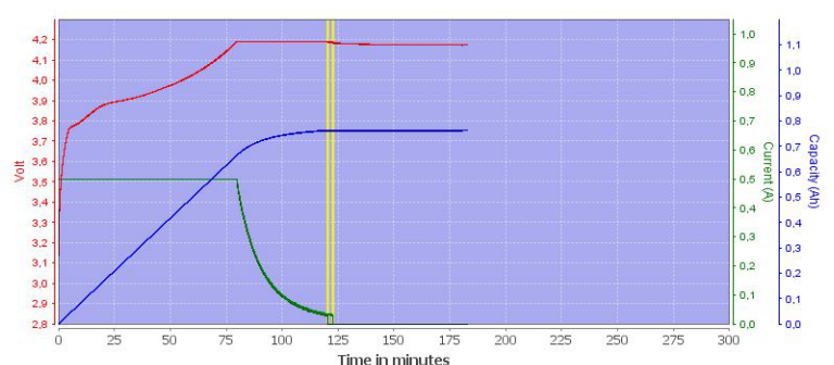
Characteristics of charging the cell ICR14650-110PCM
