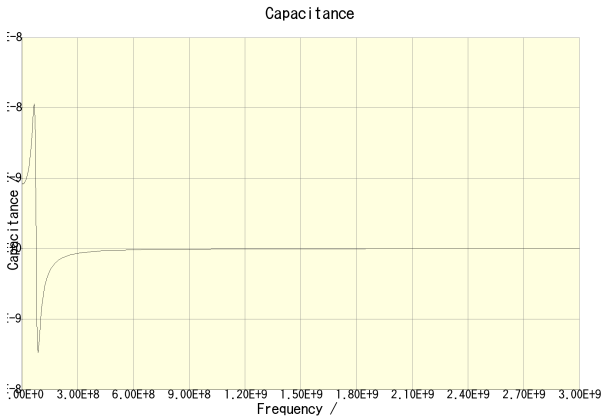
C2012X7R2E472K085AA
