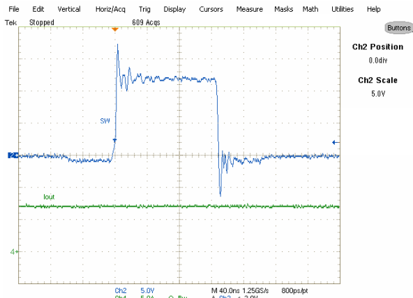
Fig. 11: Inductor node at 7A load, V_p: 0.6V , Ch_2: L_X , Ch_4: I_{out}
