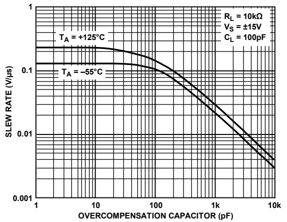
Figure 24. Slew Rate vs. Overcompensation
