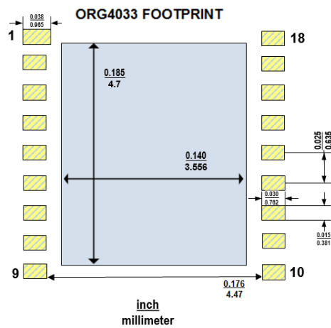
FIGURE 10 – FOOTPRINT
