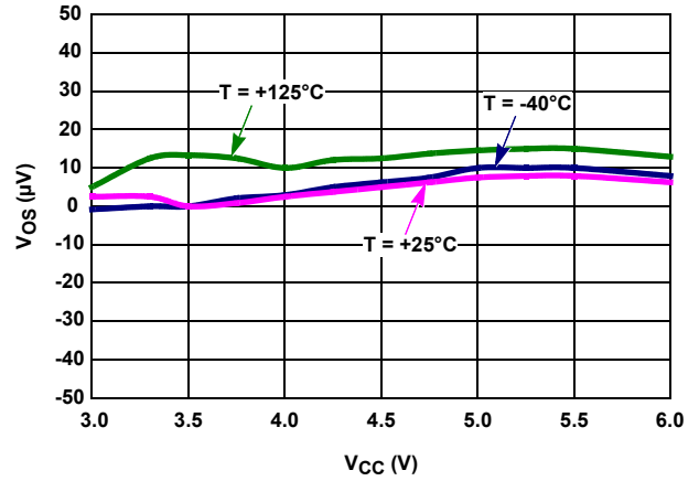
FIGURE 4. PRIMARY V_{SHUNT} V_{OS} vs V_{CC}
