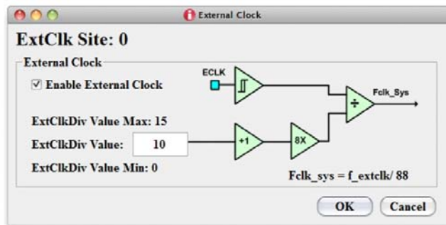
FIGURE 113. EXTERNAL CLOCK MODE
