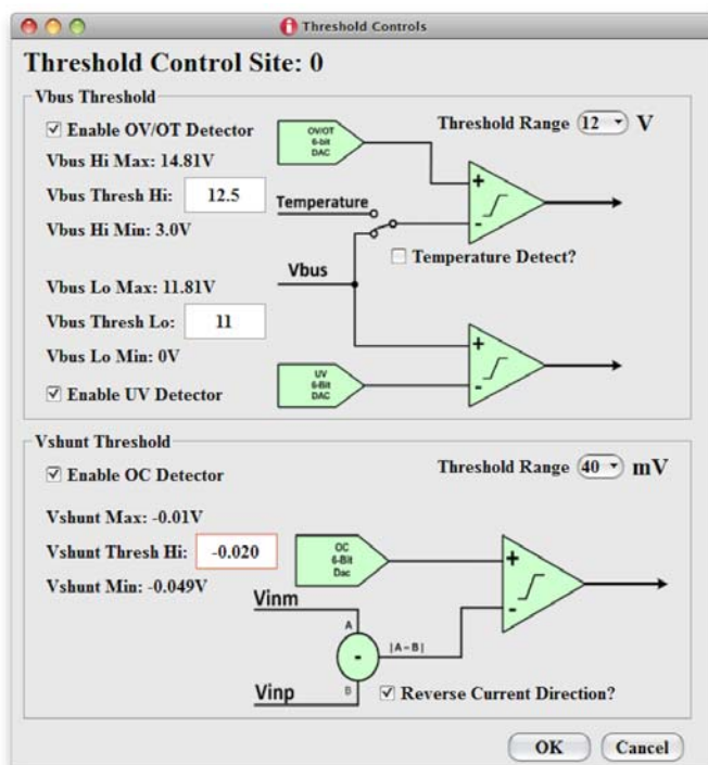
FIGURE 100. SIMPLIFIED BLOCK DIAGRAM OF THE THRESHOLD FUNCTIONS WITHIN THE DPM
