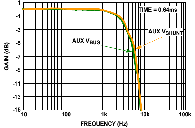
FIGURE 40. AUXILIARY V_{SHUNT} AND V_{BUS} vs FREQUENCY
