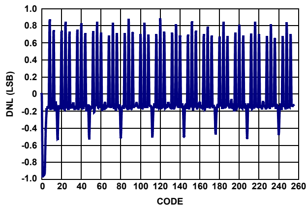
FIGURE 84. MARGIN DAC DNL
