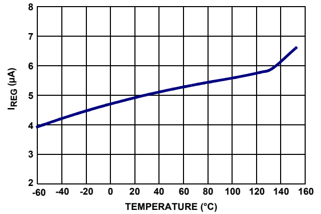
FIGURE 80. V_{REG} INPUT CURRENT vs TEMPERATURE
