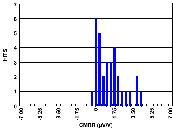
FIGURE 31. AUXILIARY V_{SHUNT} CMRR, CMV = (0V TO 3.3V)
