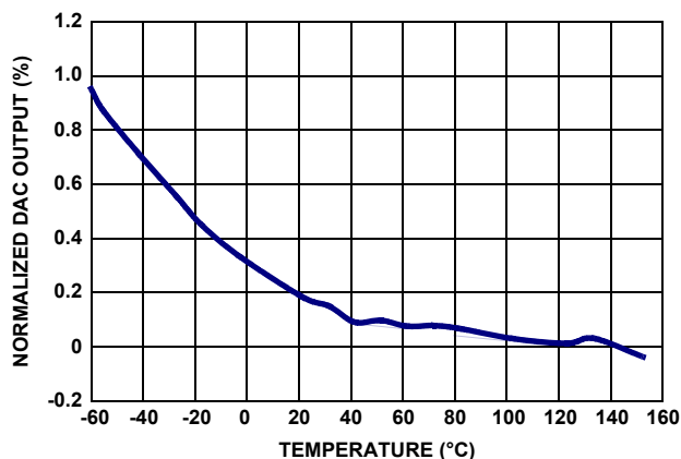
FIGURE 82. NORMALIZED DAC OUTPUT vs TEMPERATURE
