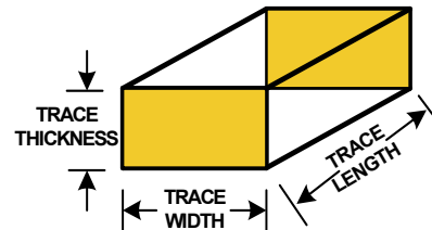
FIGURE 120. ILLUSTRATION OF THE TRACE DIMENSIONS FOR A STRIP LINE TRACE
