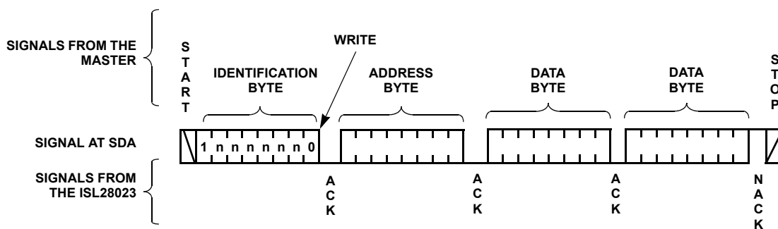
FIGURE 106. BYTE WRITE SEQUENCE (SLAVE ADDRESS INDICATED BY nnnnnn)
