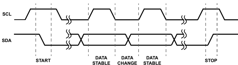
FIGURE 104. VALID DATA CHANGES, START AND STOP CONDITIONS
