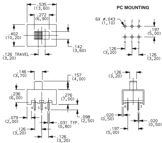
OS202013MT8QN1 DPDT
