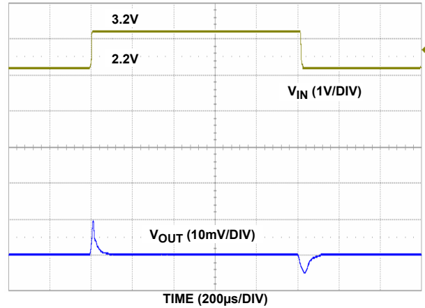
FIGURE 34. LINE TRANSIENT
