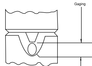
Non-Insulated Terminals
