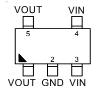
SOT-23-5 (L-Type)
