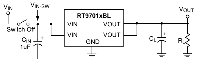
Test Circuit 2
