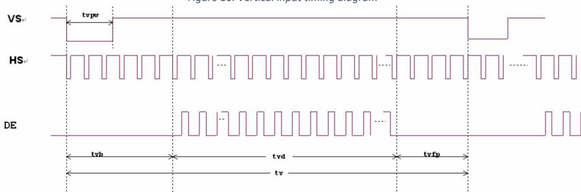
Figure 10. Vertical input timing diagram
