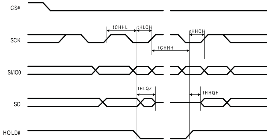
Figure 9.5 Hold Timing
