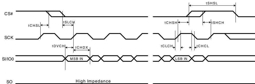
Figure 9.4 Input Timing
