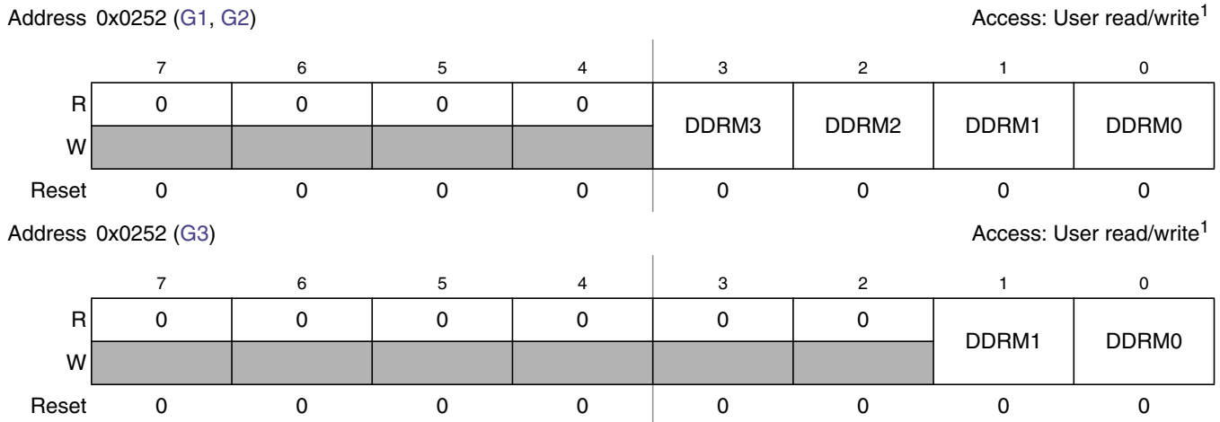
Figure 2-30. Port M Data Direction Register (DDRM)
