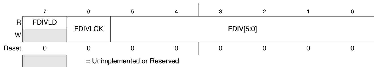
Figure 23-5. Flash Clock Divider Register (FCLKDIV)
