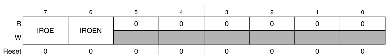
Figure 2-14. IRQ Control Register (IRQCR)
