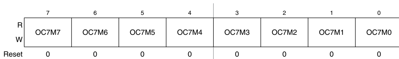
Figure 20-8. Output Compare 7 Mask Register (OC7M)
