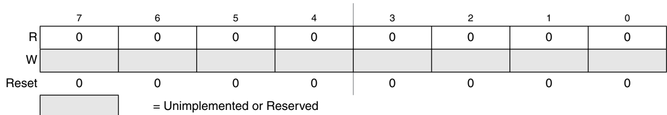
Figure 21-8. Flash Reserved0 Register (FRSV0)
