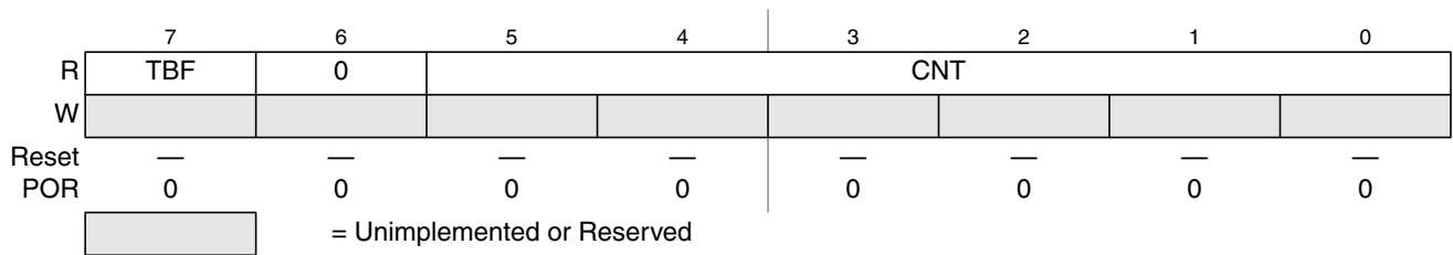
Figure 8-8. Debug Count Register (DBGCNT)
