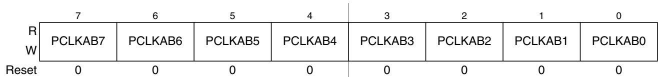
Figure 17-9. PWM Clock Select Register (PWMCLKAB)
