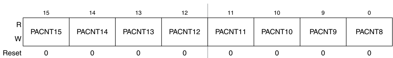
Figure 20-26. Pulse Accumulator Count Register High (PACNTH)
