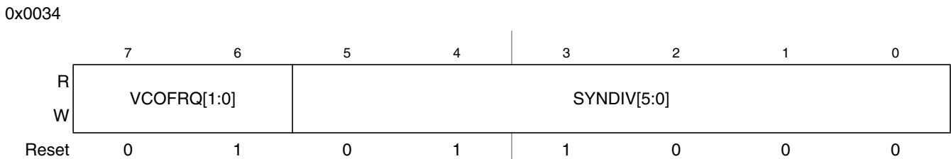
Figure 10-4. S12CPMU Synthesizer Register (CPMUSYNR)
