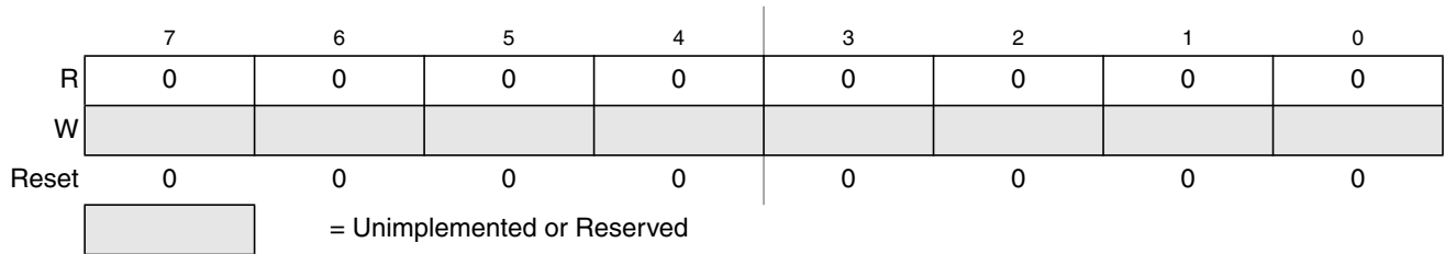
Figure 27-23. Flash Reserved5 Register (FRSV5)
