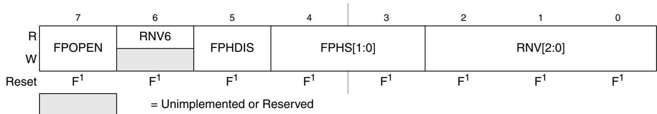
Figure 21-13. Flash Protection Register (FPROT)
