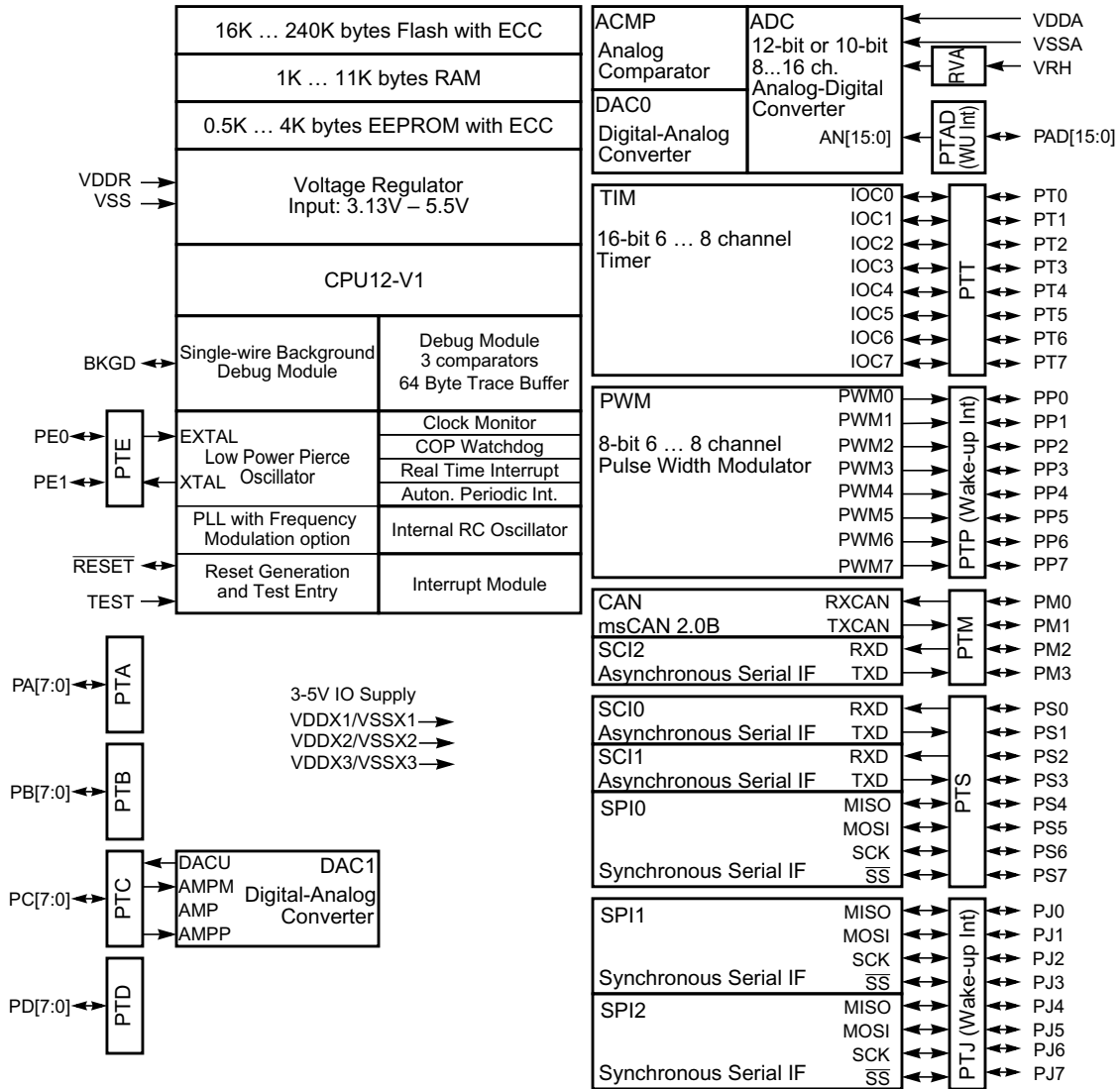
Block Diagram shows the maximum configuration! Not all pins or all peripherals are available on all devices and packages. Rerouting options are not shown.
