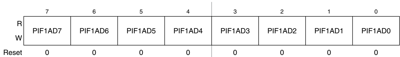
Figure 2-63. Port AD Interrupt Flag Register (PIF1AD)
