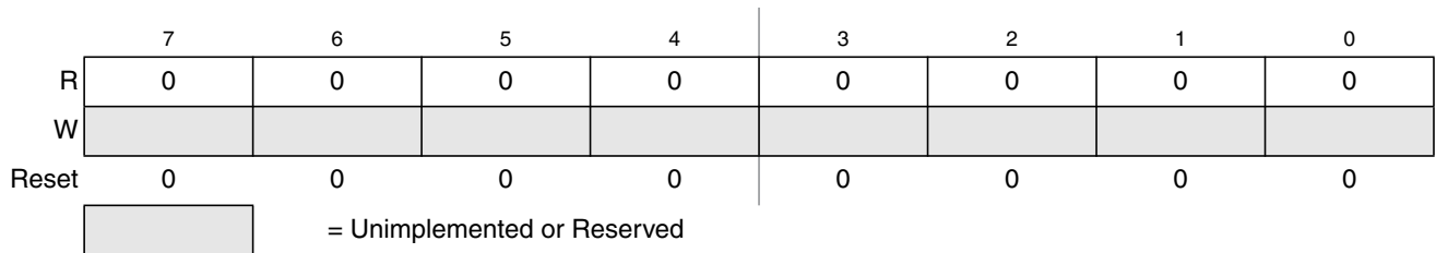
Figure 27-24. Flash Reserved6 Register (FRSV6)
