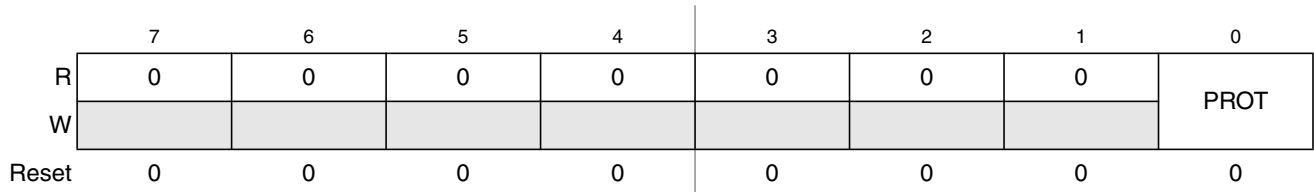
Figure 10-28. S12CPMU Protection Register (CPMUPROT)
