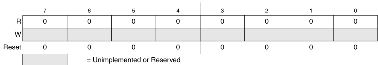
Figure 22-8. Flash Reserved0 Register (FRSV0)
