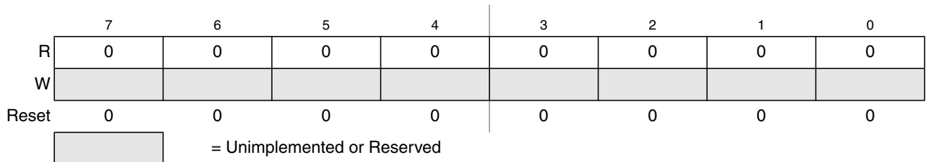
Figure 23-8. Flash Reserved0 Register (FRSV0)
