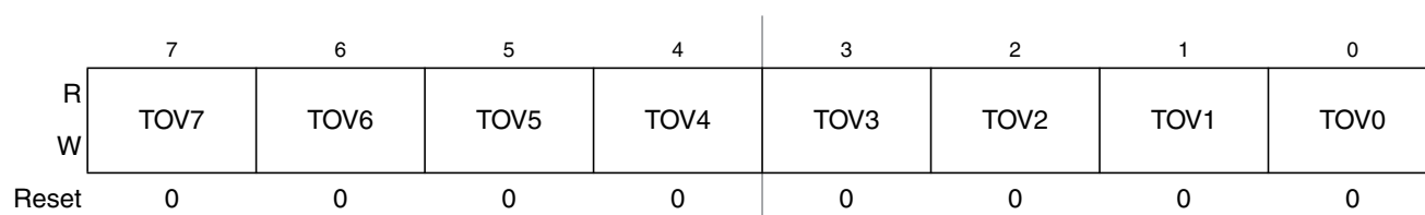
Figure 20-13. Timer Toggle On Overflow Register 1 (TTOV)
