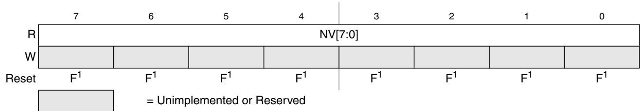
Figure 21-21. Flash Option Register (FOPT)
