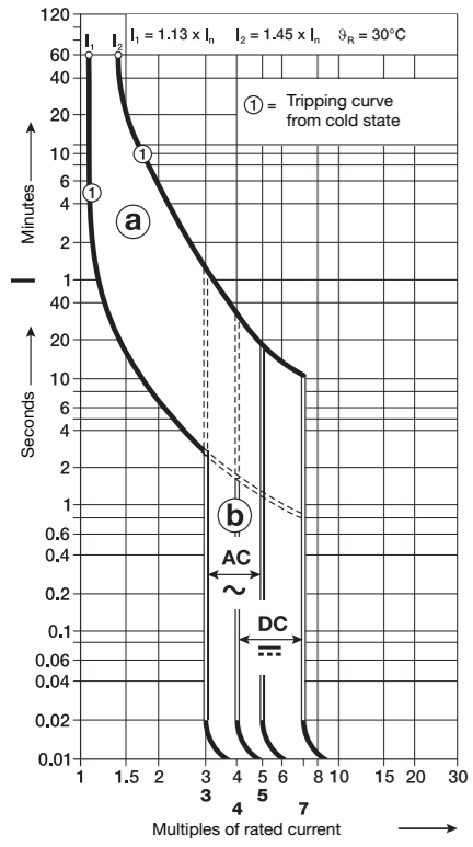
Characteristic B IEC-EN60898
