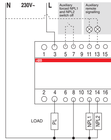
Single-phase wiring diagram
