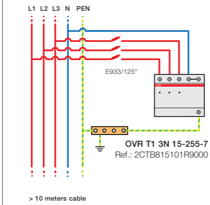
Configuration 3 I_p \leq 7 \text{ kA}
