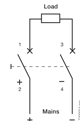
Connection diagram, two-pole (max. 250 V=) S402M-UCZ
