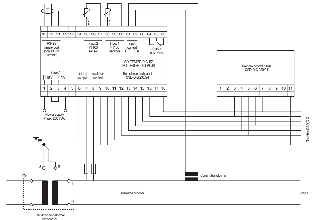
ISOLTESTER-DIG, QSD-DIG and SELVTESTER-24 -
