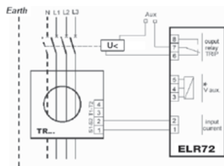
ELR72 - undervoltage release wiring
