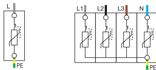
OVR T2 40 275 OVR T2 15 275
