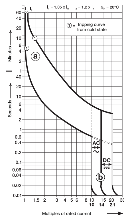
10 Characteristic K IEC-EN60947-2
