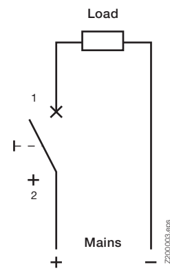
Connection diagram, single-pole (max. 125 V=) S401M-UCC
