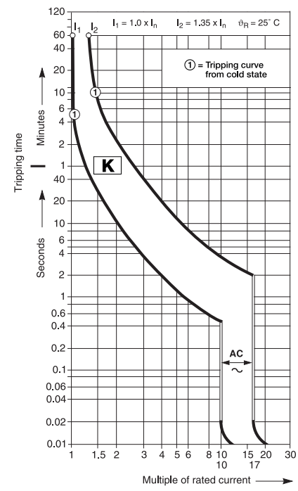
Characteristic K S 200 U/S 200 UP/SU 200 PR
