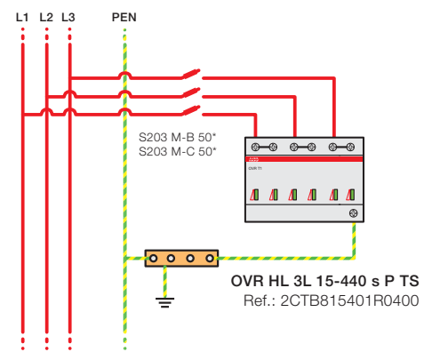
Configuration 1 I_p \leq 50 \text{ kA}
