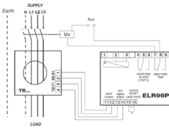
ELR96P - undervoltage release wiring
