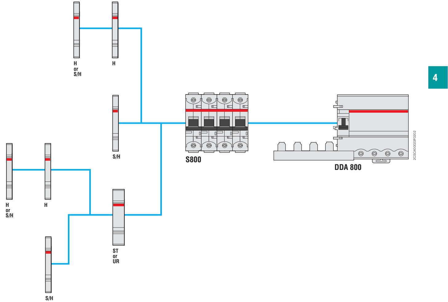
Combination between auxiliary elements and S800
