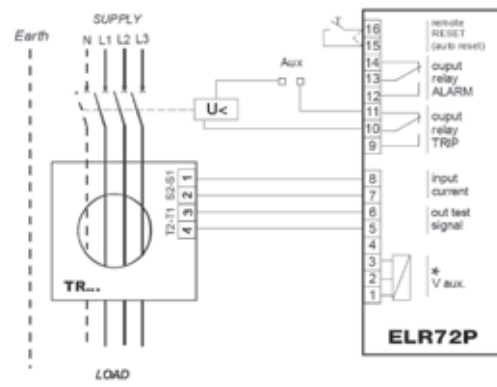
ELR72P - undervoltage release wiring
