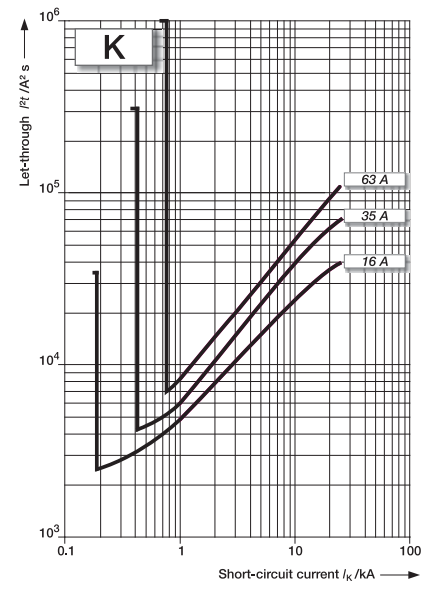
S 750 DR characteristic K_{selective} diagram of let-through values I^2t 16... 63 A
