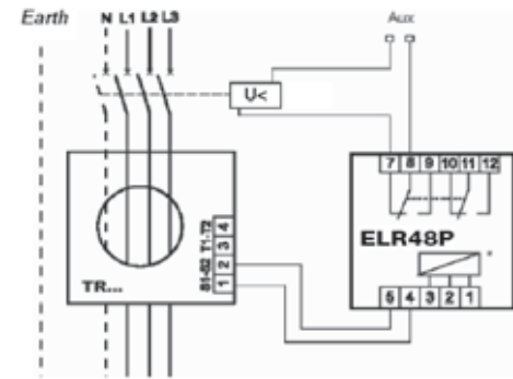
ELR48P - undervoltage release wiring
