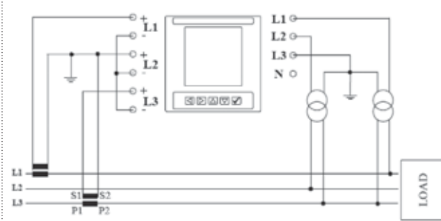
Insertion with 2 CTs and 2 VTs (Aron)
