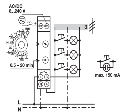
E 232E-8/230 Multi 10 3 conductor
