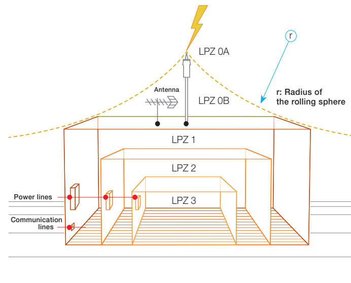
External lightning protection system
