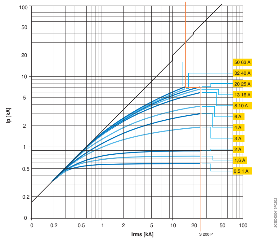
S 200-S 200 M-S 200 P, characteristic Z
