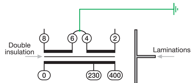
Lamination not grounded Connection 12-0-12 preserving double insulation
