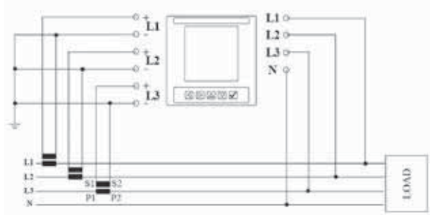
Insertion with 3 CTs
