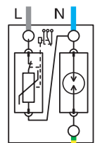
OVR T2 1N 15 275 P TS OVR T2 1N 40 275 P TS
