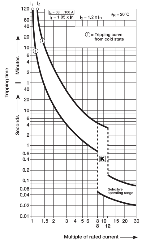
Characteristic K selective S 700 - 63 ... 100 A
