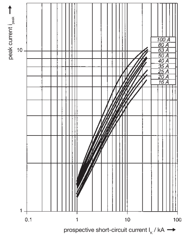
S 700 characteristic K_{selective} let-through peak current ( I_{peak} )
