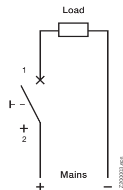
Connection diagram, single-pole (max. 125 V=) S401M-UCZ
