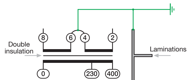
Lamination grounded The insulation between the primary and secondary is reduced to that between the laminations and primary. Consequently, this assembly takes away the advantage of double insulation.
