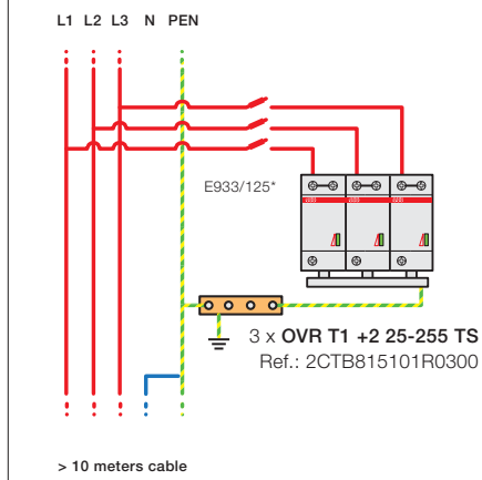
Configuration 2 7 \text{ kA} \leq I_p \leq 15 \text{ kA}
