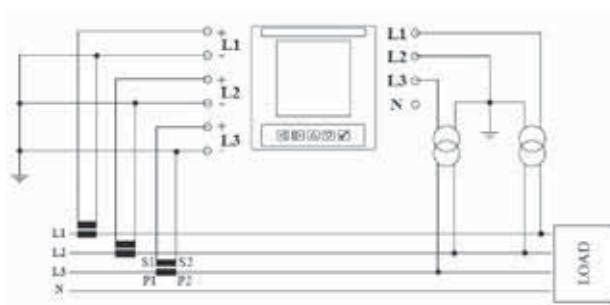
Insertion with 3 CTs and 2 VTs
