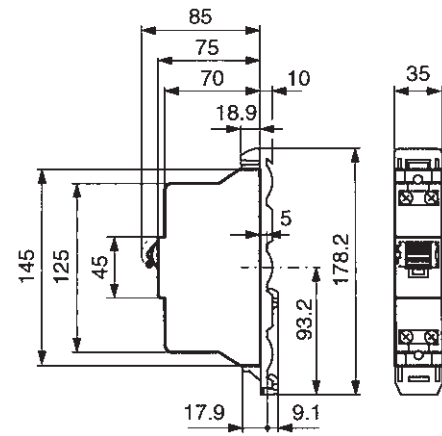
S 701 with DIN rail adapter
