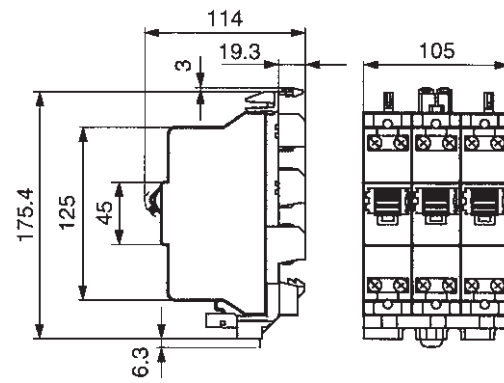
3 x S 701 with busbar adapter
