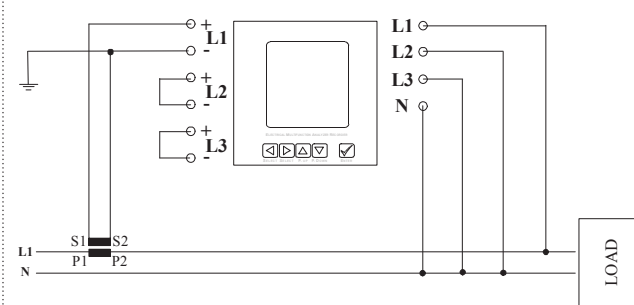
Single phase insertion with 1CT
