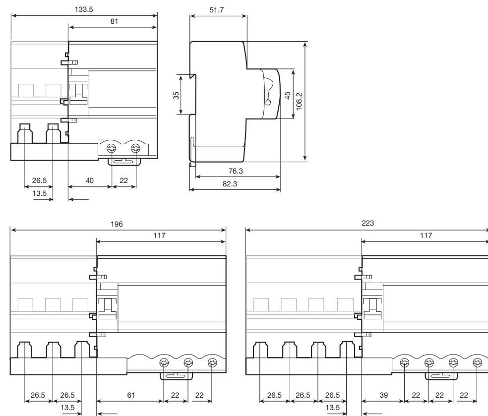
DDA 800 for S800 and DS800 series
