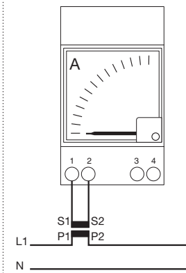
Indirect insertion using C.T.
