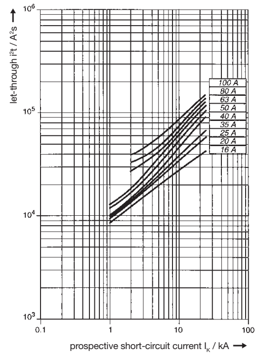
10 S 700 characteristic K_{selective} let-through energy
