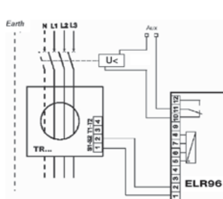
ELR96 - undervoltage release wiring
