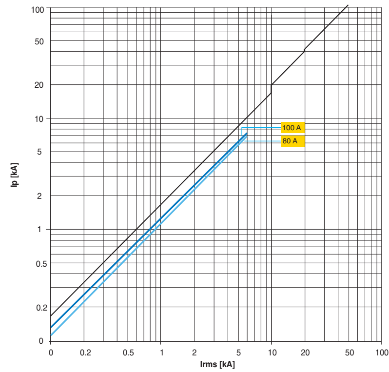
S 280 80-100 A, characteristic B
