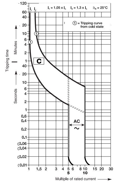
Characteristic C S 200 U/S 200 UP
