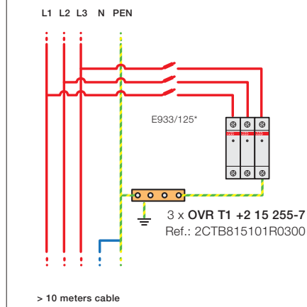
Configuration 3 I_p \leq 7 \text{ kA}
