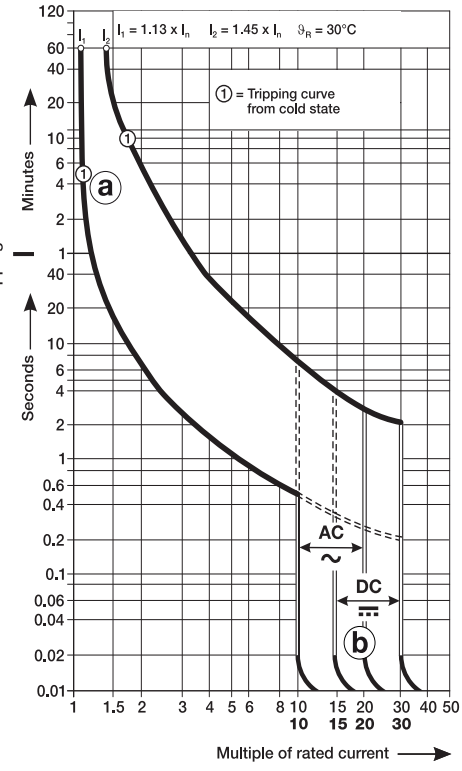
Characteristic D IEC-EN60898
