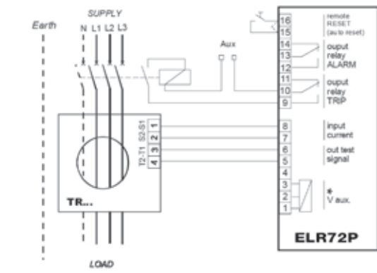
ELR72P - shunt trip wiring
