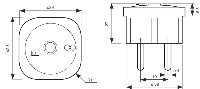
LEE 230 power failure signalling lamp
