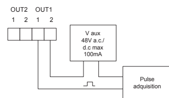
Digital output used as pulses
