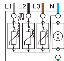
OVR T2 3N 15 275 P TS OVR T2 3N 40 275 P TS
