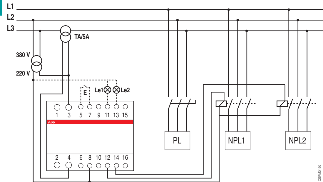
Balanced three-phase wiring diagram
