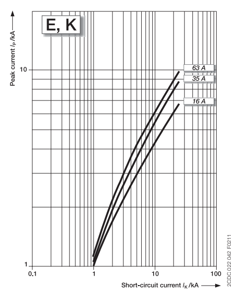
S 750 DR characteristic E_{selective} \cdot K_{selective} let-through peak current ( I_{peak} )
