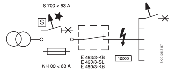
E463 / E480 Short-circuit withstand capacity
