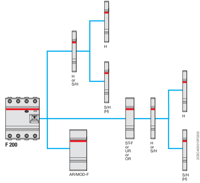
Combination of auxiliary elements with F 200
