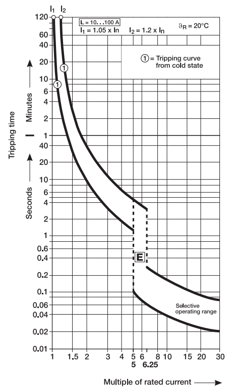
Characteristic E selective S 750 DR - 16 ... 25 A
