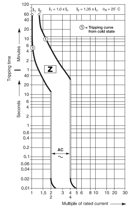
Characteristic Z S 200 U/S 200 UP
