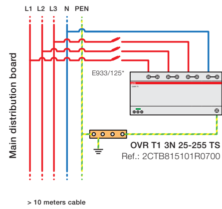
Configuration 1 15 \text{ kA} \leq I_p \leq 50 \text{ kA}
