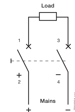
Connection diagram, two-pole (max. 250 V=) S402M-UCC
