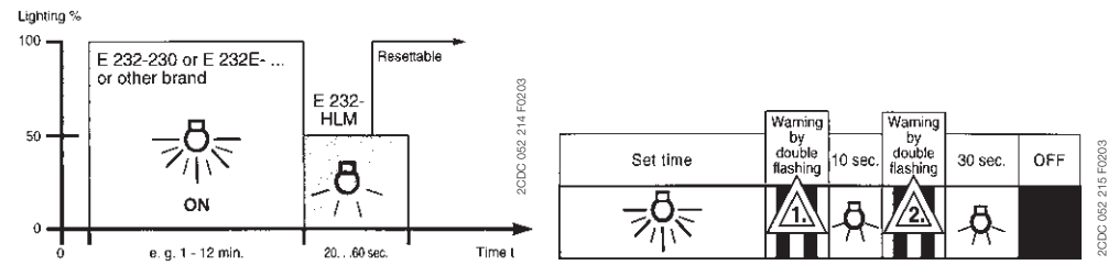
timing of a staircase lighting time-delay switch with semi-light module E 232-HLM
