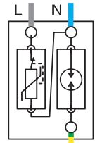
OVR T2 1N 15 275 P OVR T2 1N 40 275 P
