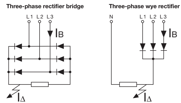
Phase currents
