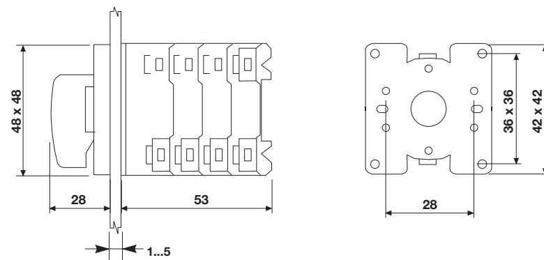
QCV - QCA front panel voltmetric and ammetric switches
