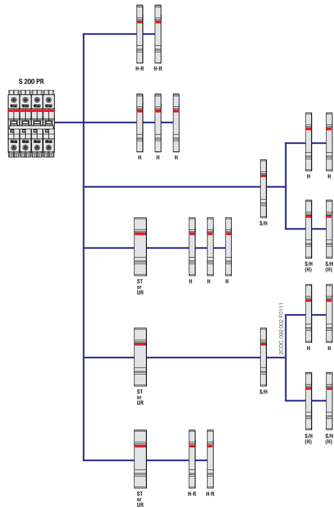
Combination of auxiliary elements with SU 200 PR
