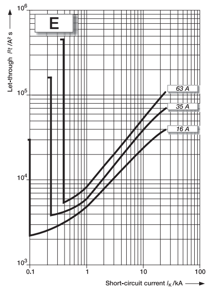
S 750 DR characteristic E_{selective} diagram of let-through values I^2t 16... 63 A
