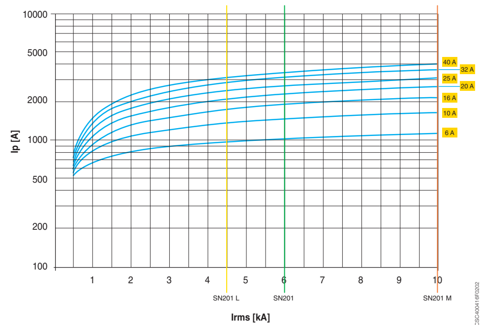
10 SN 201 L, SN 201, SN 201 M, characteristic B 230 V
