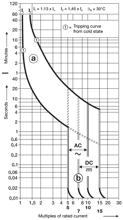
Characteristic C IEC-EN60898
