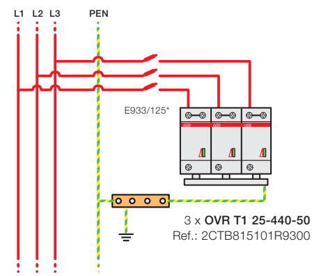
Configuration 2 I_p \leq 15 \text{ kA}
