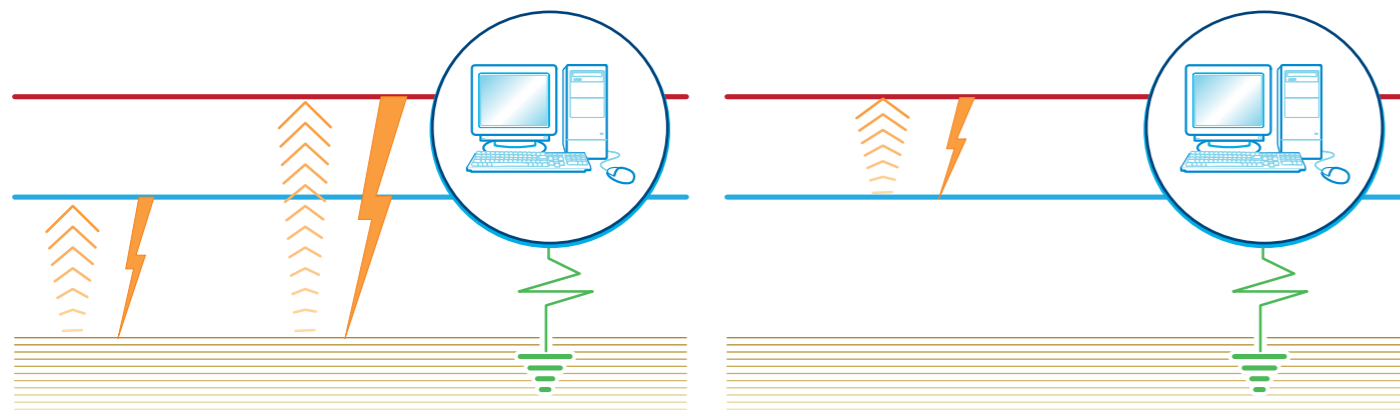
Overvoltages in common mode
