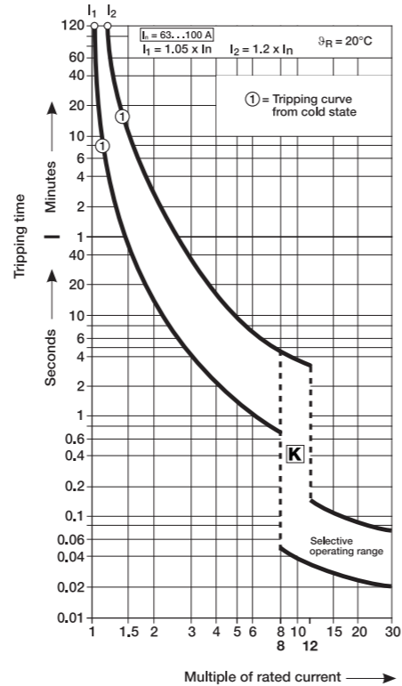
Characteristic K selective S 700 - 63 ... 100 A
