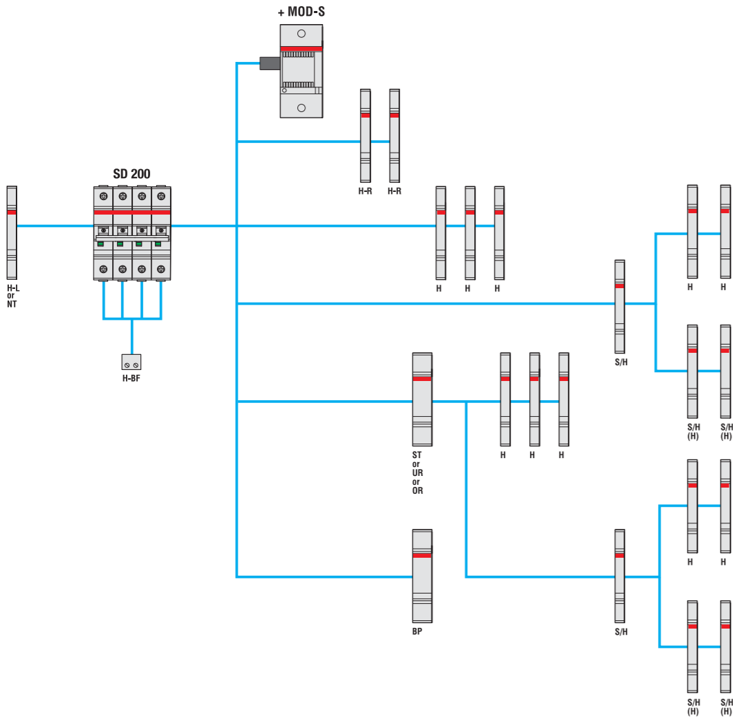
Combination of auxiliary elements with SD 200
