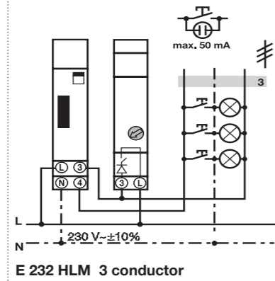
E 232 HLM 3 conductor
