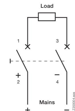
Connection diagram, two-pole (max. 250 V=) S402M-UCZ
