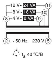
TS24/4-8-12
