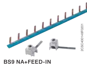
BS9 NA+FEED-IN
