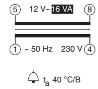
TS16/4-8-12
