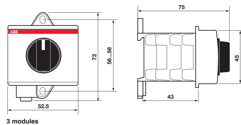
MCV - MCA voltmetric and ammetric switches
