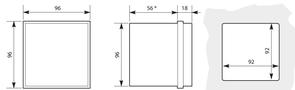
ELR96
