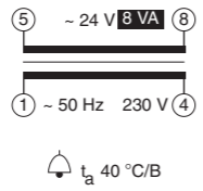
TS8/4-6-8 SW
