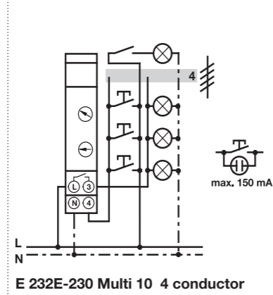
E 232E-230 Multi 10 4 conductor
