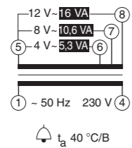
TS16/4-8-12
