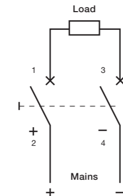
Connection diagram, two-pole (max. 250 V=) S402M-UCC
