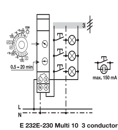
E 232E-230 Multi 10 3 conductor
