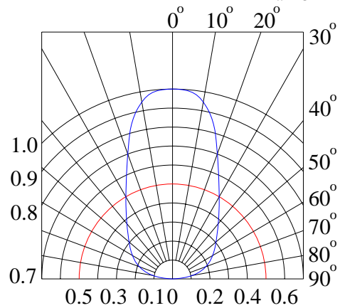
Radiation Diagram
