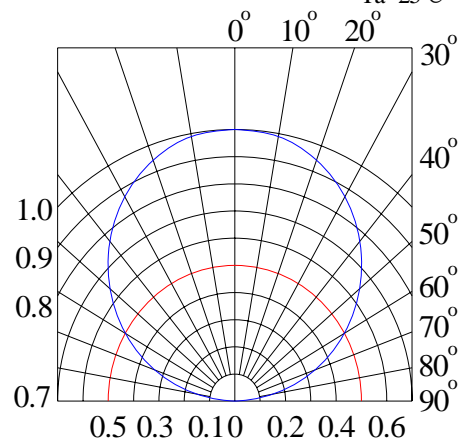
Radiation Diagram
