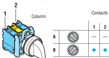
Contact activation of 2-position selector switch
