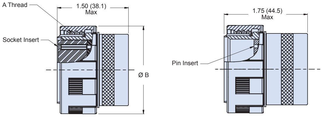
06 Plug Adapter U.S. PATENT NO. 5,960,137
