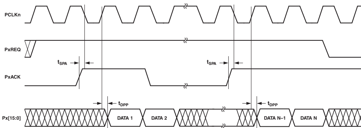
Figure 15. Slave Mode PxAck to PCLKn Switching Characteristics (n = 0 and x = A, B; or n = 1 x = C, D)
