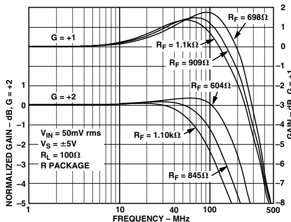
Figure 8. R_{FEEDBACK} vs. Frequency Response, G = +1/+2
