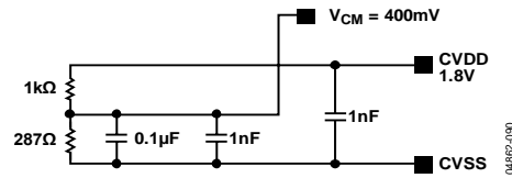
Figure 92. DACCLK V_{CM} Generator Circuit
